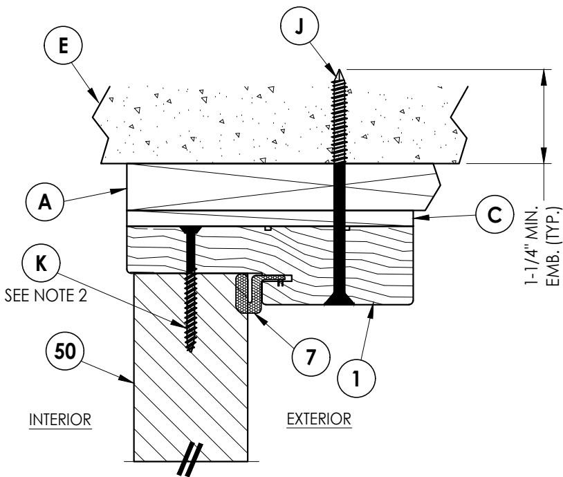
4 VERTICAL CROSS SECTION Inswing Shown (Outswing Similar) 1X Buck Construction
