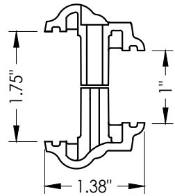
3A ODL LITE FRAME HP Polypropylene
