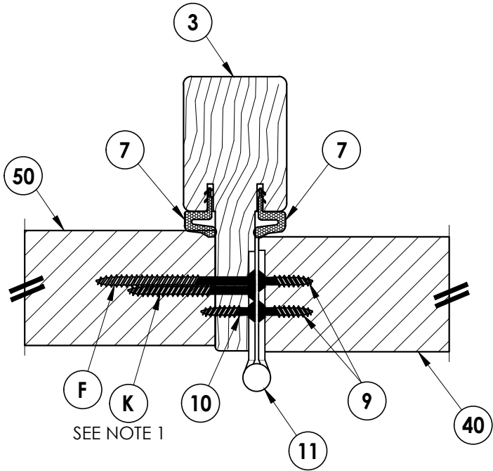
1 HORIZONTAL CROSS SECTION 8 Inswing Shown (Outswing Similar)
