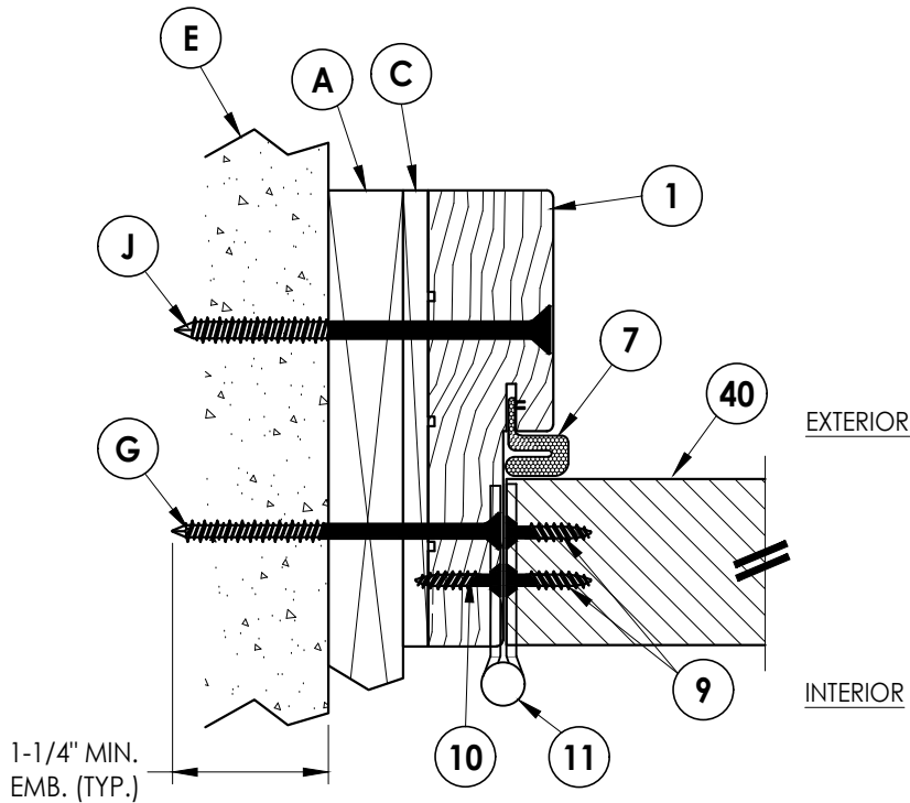
1 HORIZONTAL CROSS SECTION Inswing Shown (Outswing Similar) 1X Buck Construction
