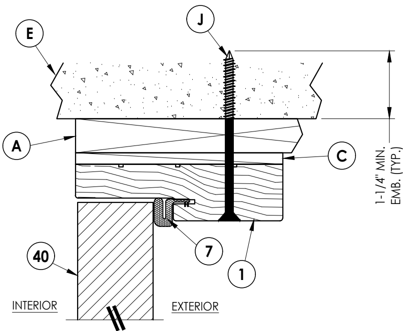
3 VERTICAL CROSS SECTION Inswing Shown (Outswing Similar) 1X Buck Construction
