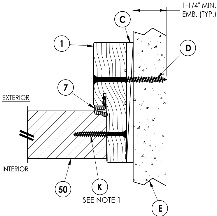
2 HORIZONTAL CROSS SECTION Inswing Shown (Outswing Similar) Shown Direct to Masonry
