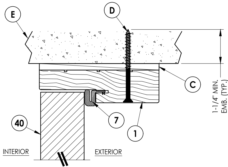
3 VERTICAL CROSS SECTION Inswing Shown (Outswing Similar) Shown Direct to Masonry
