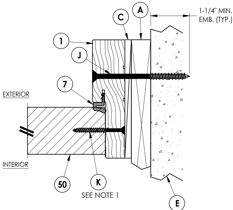
2 HORIZONTAL CROSS SECTION Inswing Shown (Outswing Similar) 1X Buck Construction
