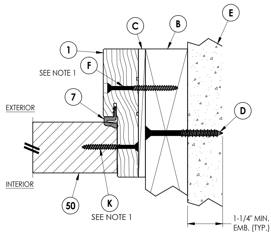
2 5 HORIZONTAL CROSS SECTION Inswing Shown (Outswing Similar) 2X Buck Construction
