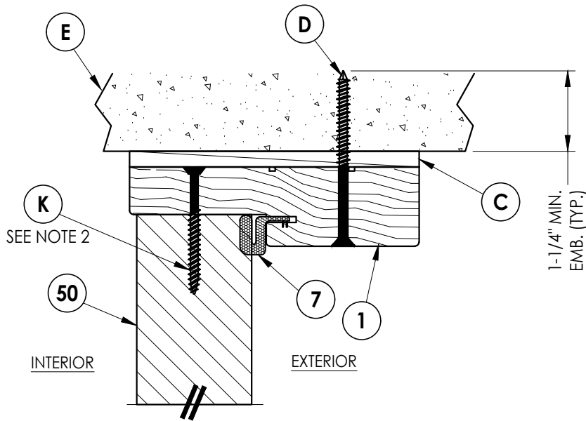
4 VERTICAL CROSS SECTION Inswing Shown (Outswing Similar) Shown Direct to Masonry
