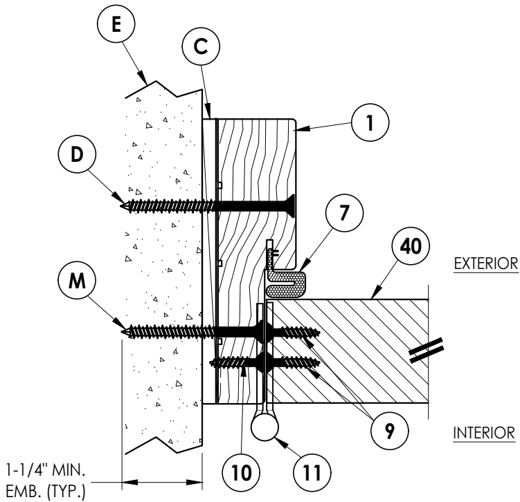
1 HORIZONTAL CROSS SECTION Inswing Shown (Outswing Similar) Shown Direct to Masonry
